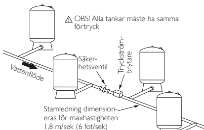
Fig. I.5 Multitankinstallation
