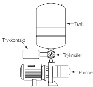
Fig. 1.4-5 Booster pumpe m/ inline tank
